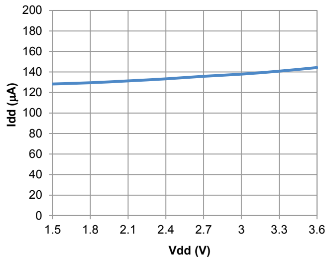
Figure 5: Typical Idd vs Vdd
